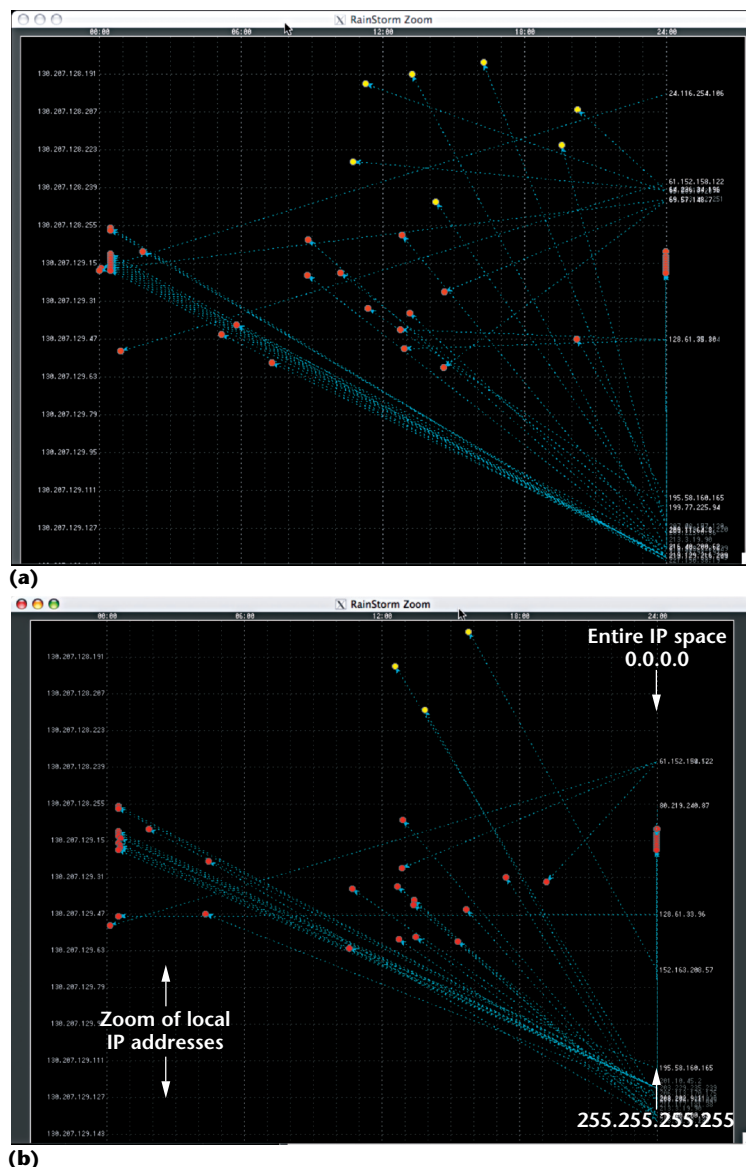
3 Botnet activity shown in a zoom view for the same IP address space on (a) 26 April 2005 and (b) 27 April 2005. (Botnets are groups of compromised computers that are under the command and control of a malicious entity.) Internal IP addresses appear on the left vertical axis and external IP addresses are on the right vertical axis. The activity time pattern for the two days is almost identical.
