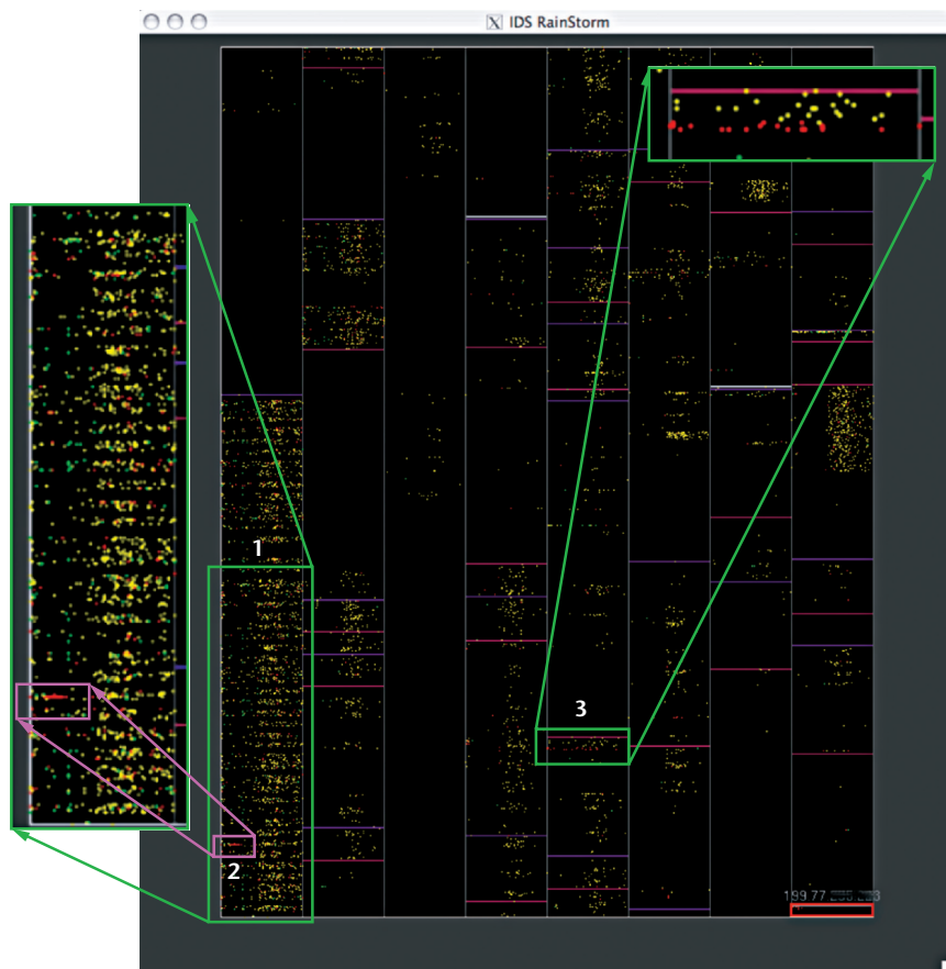
5 Overview of alarms on 27 April 2005. (Two regions are artificially identified in green and magnified for easier viewing.) Region 1 shows activity in a subset of campus dorm IP addresses. Region 2 outlines a cluster of activity for a machine in the dorm. Region 3 shows a cluster of activity occurring over a small range of IP addresses for the entire day.
