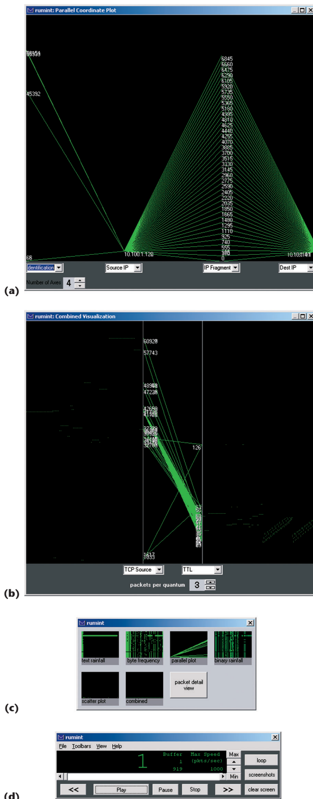
6 Overview of the Rumint packet visualization system. Each window provides specialized insight into network traffic and can be used alone or in combination. (a) Parallel coordinate-plot display, (b) glyph-based animation display, (c) thumbnail toolbar, and (d) personal video recorder interface.
